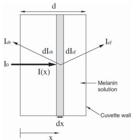
FIGURE 2 Cuvette geometry.
